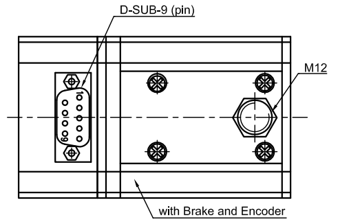
Top view A
