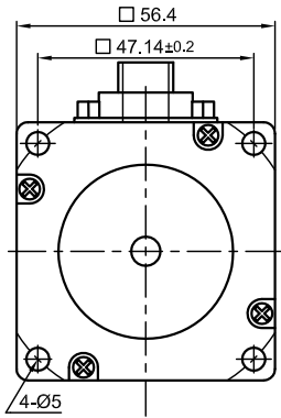
Front view and mounting
